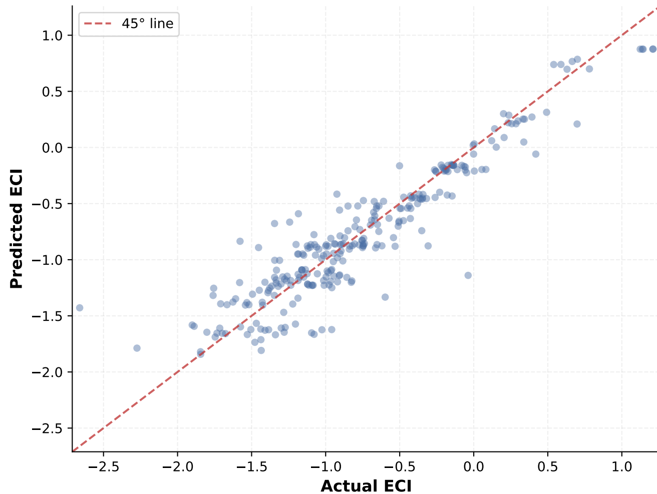
Random Forest — ECI | Test R^2=0.864 RMSE=0.2404
