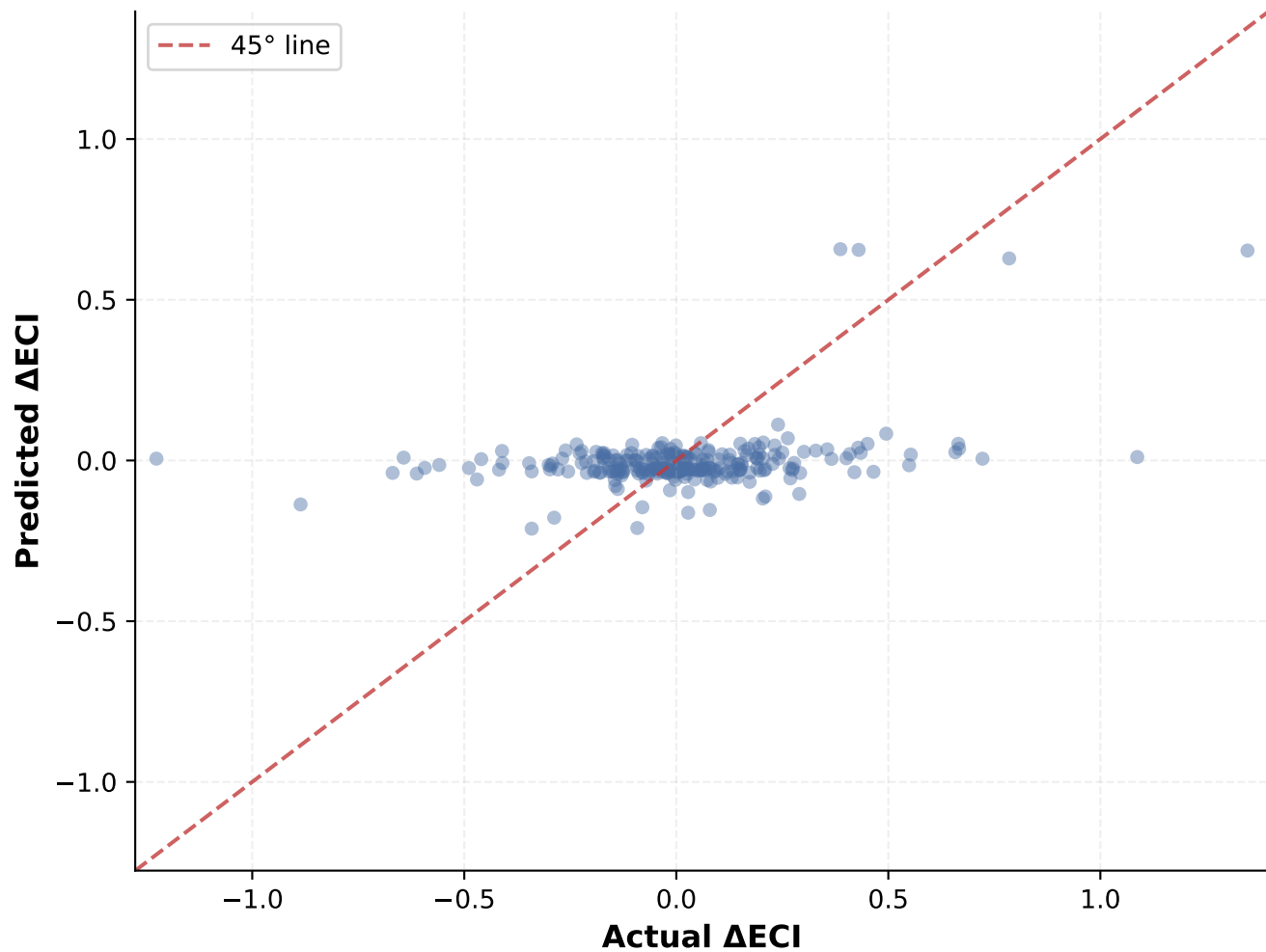
Random Forest — \Delta ECI | Test R^2=0.148 RMSE=0.2403
